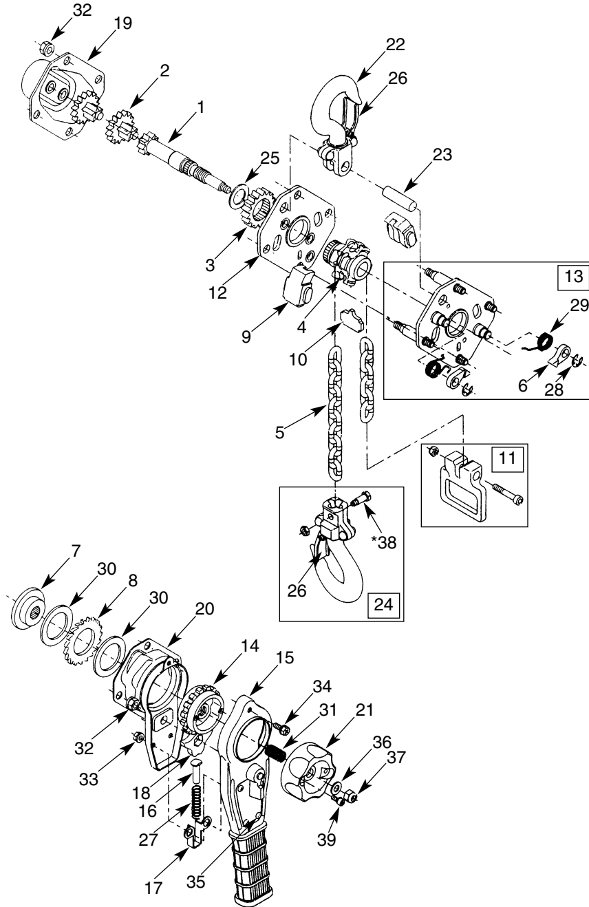
Figure 15 - .75 & 1.5 Ton Models
